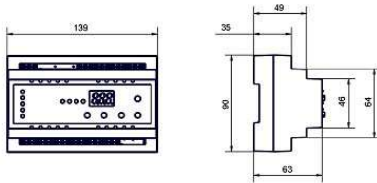
Figure 3.1 – TR-101 dimensions
